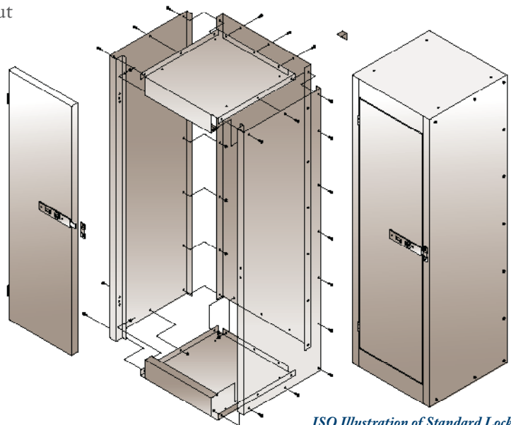
ISO Illustration of Standard Locker
